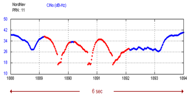
Figure 14. Example of Frequent Deep Fades
