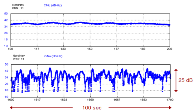
Figure 1. Example of Deep Signal Fading due to Ionospheric Scintillation
